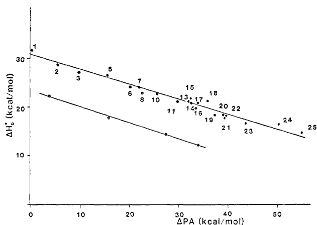
Figure 5. Correlation between \Delta H^\circ_{\text{D}} and \Delta\text{PA} for -\text{OH}^+\cdots\text{OH}_2 dimers (●, upper line) and -\text{SH}^+\cdots\text{O}- dimers (○, lower line). Numbers refer to reactions in Table III.
