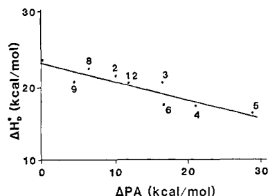
Figure 4. Correlation between \Delta H^\circ_D and \Delta PA for -\text{NH}^+\cdots\text{N}- bonds. Numbers refer to reactions in Table II. For \Delta PA = 0 , average \Delta H^\circ_D of symmetric dimers is used.
